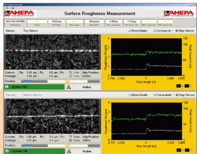
The laser line and the galvanized surface texture (here EDT) are clearly visible. The example of a screenshot shows the online Ra and R Pc results over the coil length with the most recent microscopic image. The high dynamic of the system allows the operator to quickly correct the overshoot of the roughness when changing the strip's material (in the middle of the diagram).
